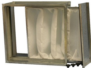
MEZ Flanged Side Access Housing (1820)
